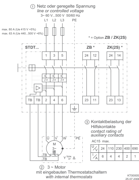
Connection diagram S-ET
