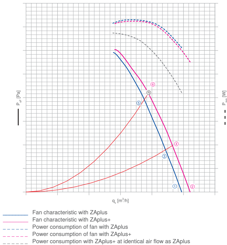
Increase in air flow rate ZApus+ vs ZApus
