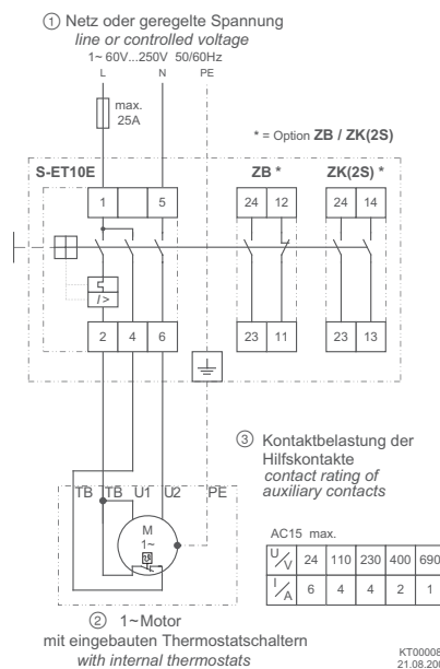
Connection diagram STDT
